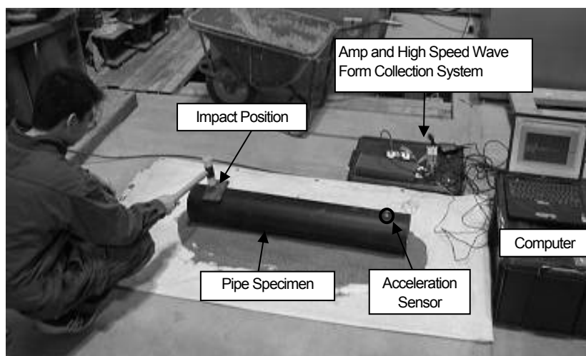
Photo-3 Impact-elastic wave method Experiment
