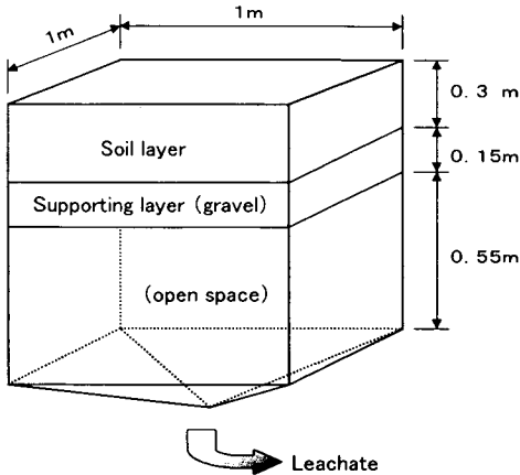
Fig. 1 Summary of inside of a lysimeter
