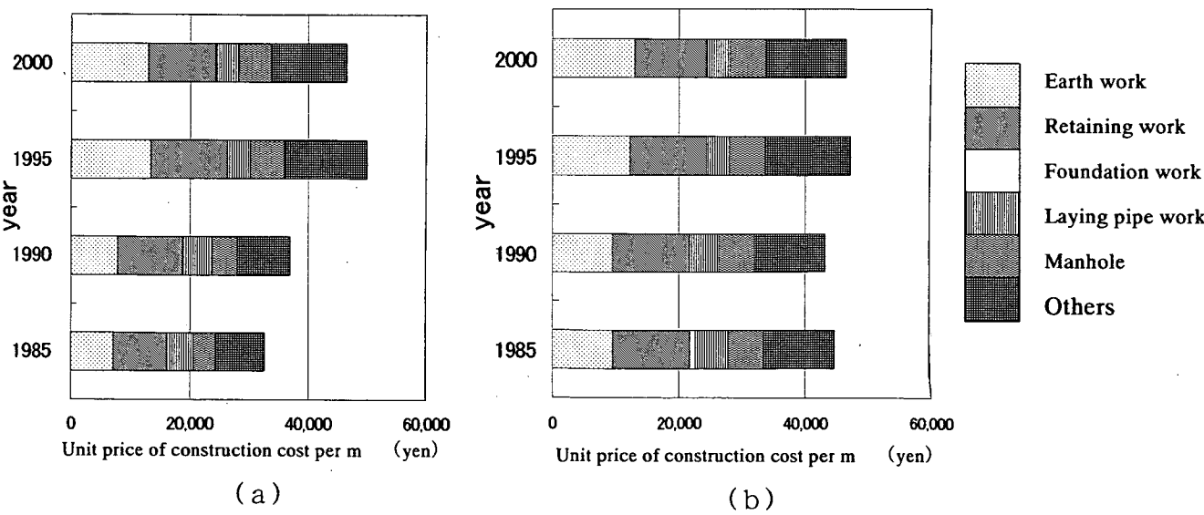
Fig.2 Cost of small pipe system by the open cut method
