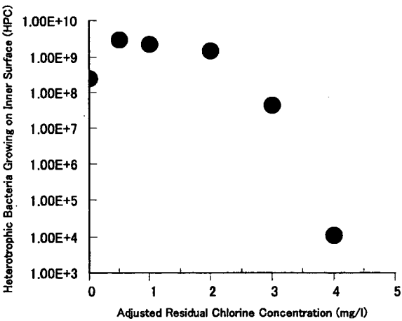
Fig. 1 Control of Adherent Heterotrophic Bacteria by Residual Chlorine
