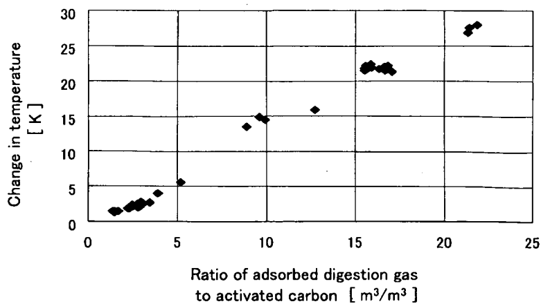
Fig. 3 Relationship between ratio of adsorbed digestion gas to activated carbon, and change in quantity with temperature
