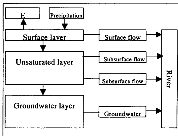
Fig.1 Water circulation flow in river basin
