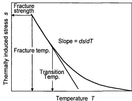
Figure 39 TSRST results
