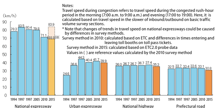
Figure 1. Changing average travel speeds during congestion periods (business days)
