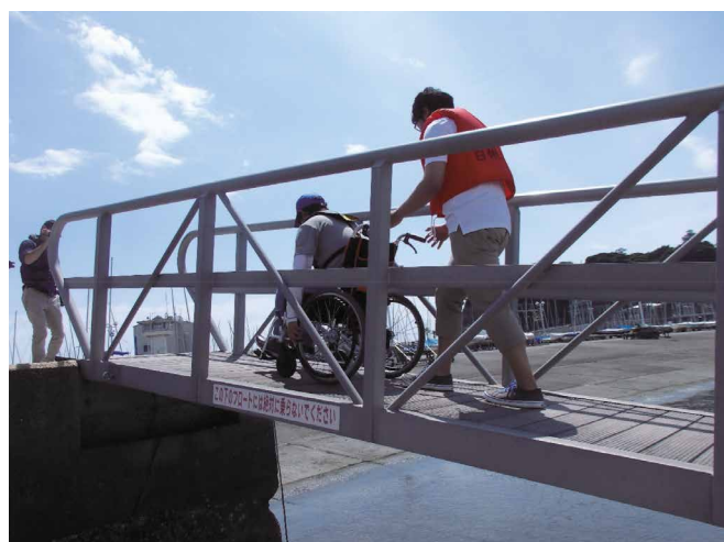
Photo Wheelchair during the proving test of a connecting bridge
